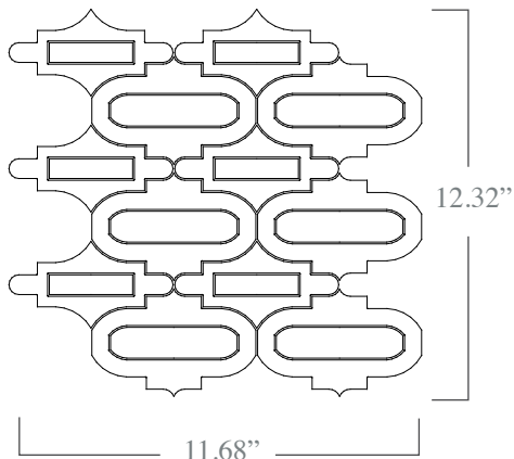
11.68" x 12.32" x 3/8 "(5 lbs) 1 sq ft per template
